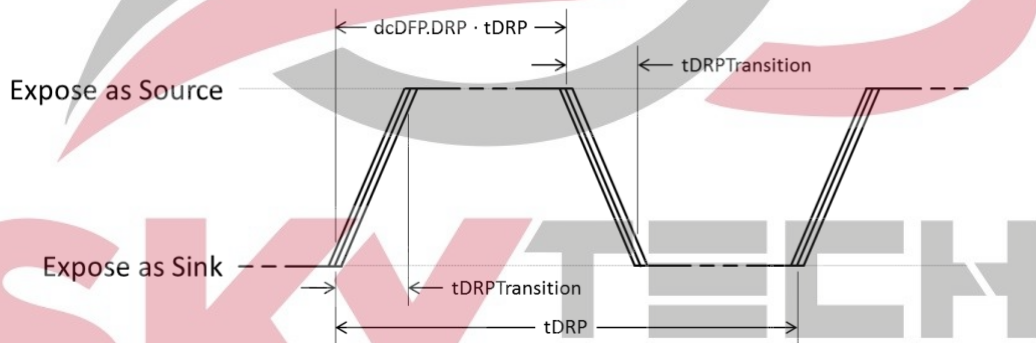
Figure 4-36 DRP Timing
